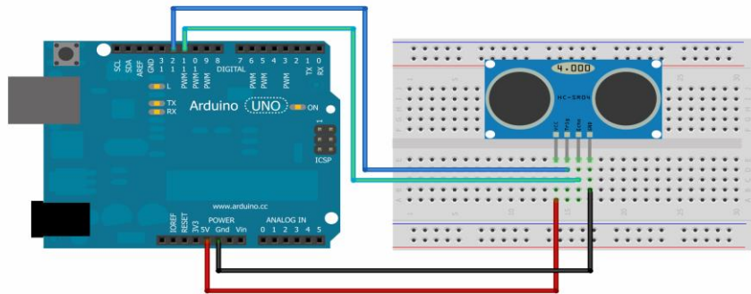
Figure 4: Hardware organization of Height Sensor
