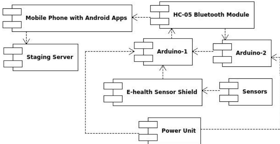
Figure 6: Portable telemedicine tool kit component diagram
