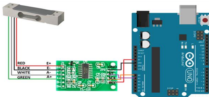
Figure 5: Hardware organization of Weight Sensor
